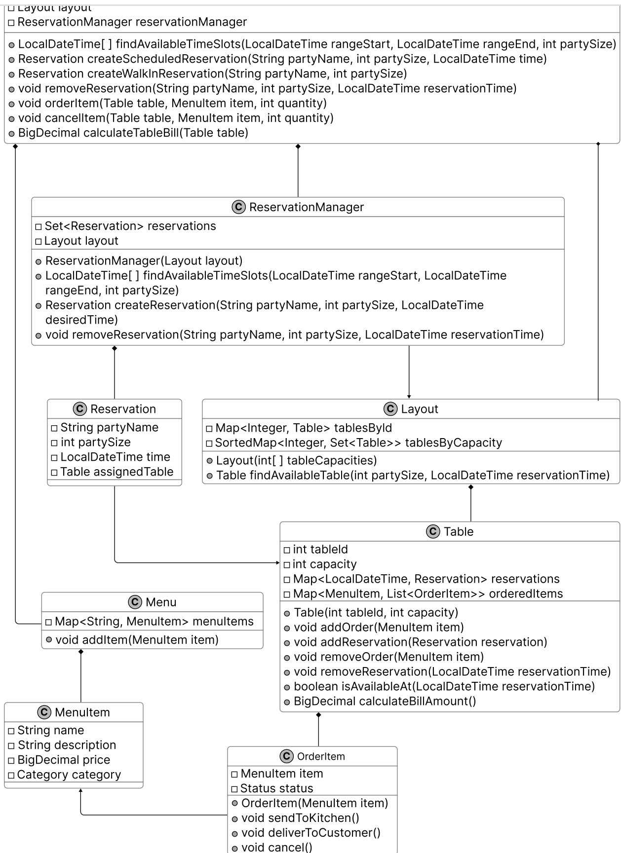
Class Diagram of Restaurant Management System
