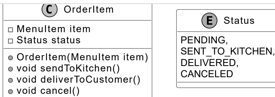
OrderItem class and Status enum
